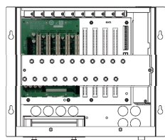
HPE-6S1 1 x CPU 4 x PCI 1 x PCI-E x4
