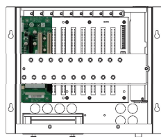
HPE-3S2 1 x CPU 1 x PCI 1 x PCI-E x4
