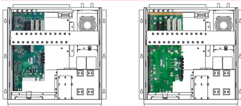
EBP-5E1 1 x PICMG CPU, 1 x PCI-E x16, 1 x PCI-X, 2 x PCI
